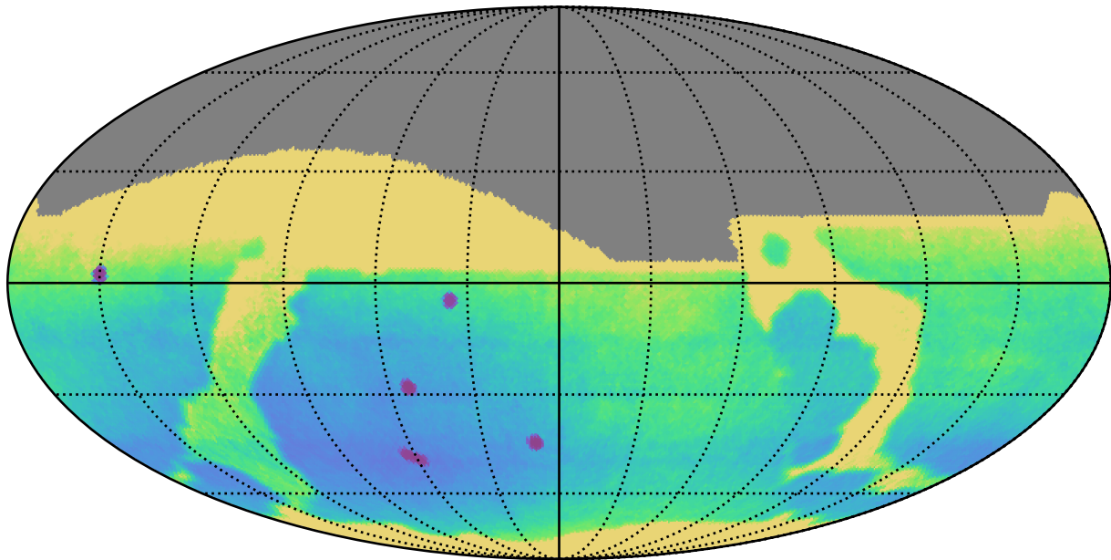
ddf_acor_sf10_lsf20_lsr20_v3.4_10yrs : Parallax Uncert @ 24.0
