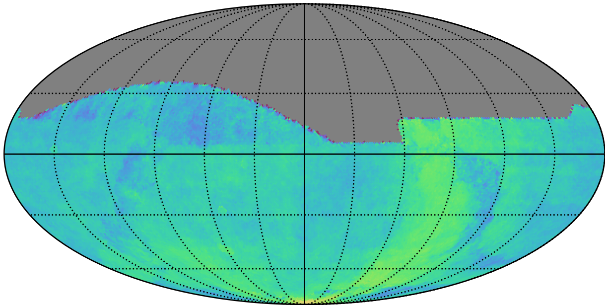
ddf_acor_sf10_lsf20_lsr20_v3.4_10yrs : Parallax Coverage @ 24.0
