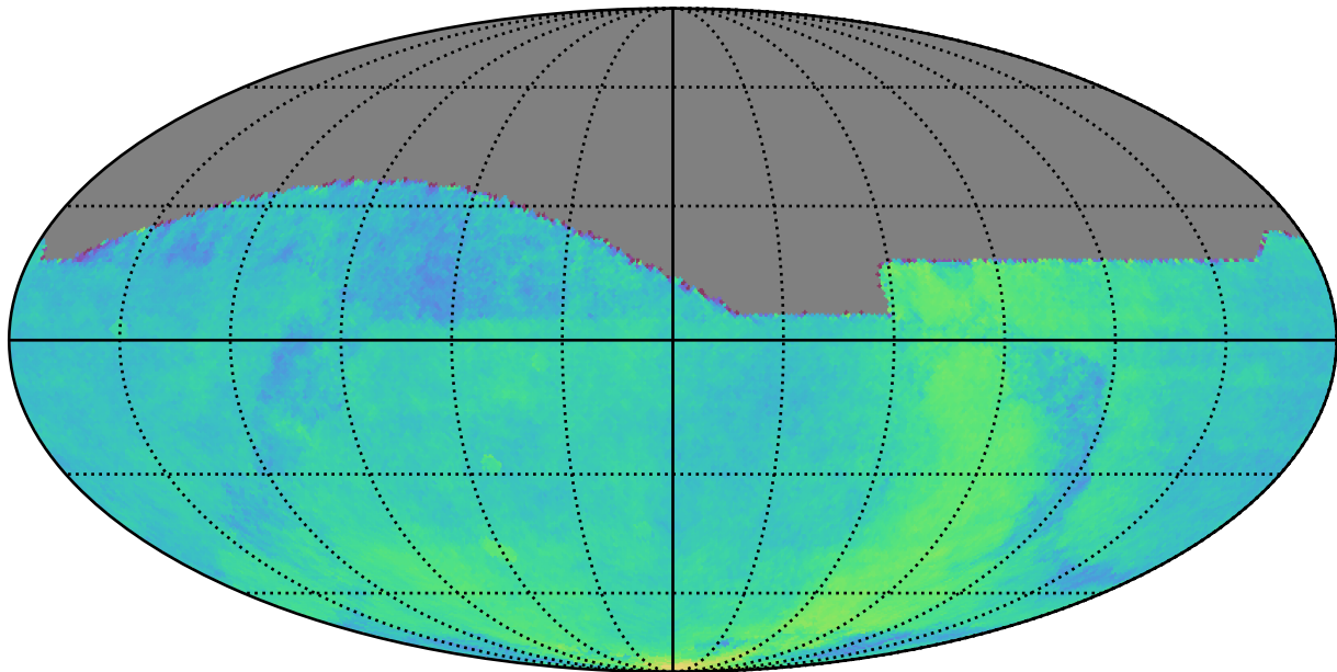
ddf_acor_sf10_lsf20_lsr20_v3.4_10yrs : Parallax Coverage @ 22.4
