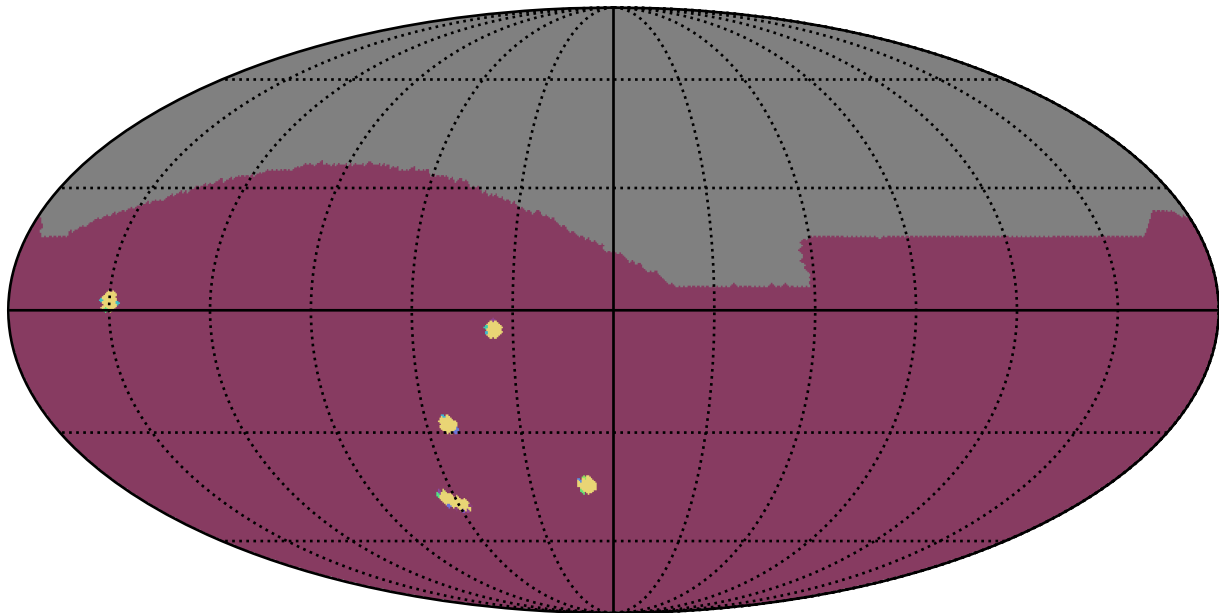
ddf_acor_sf10_lsf20_lsr20_v3.4_10yrs : NumberOfQuickRevisits
