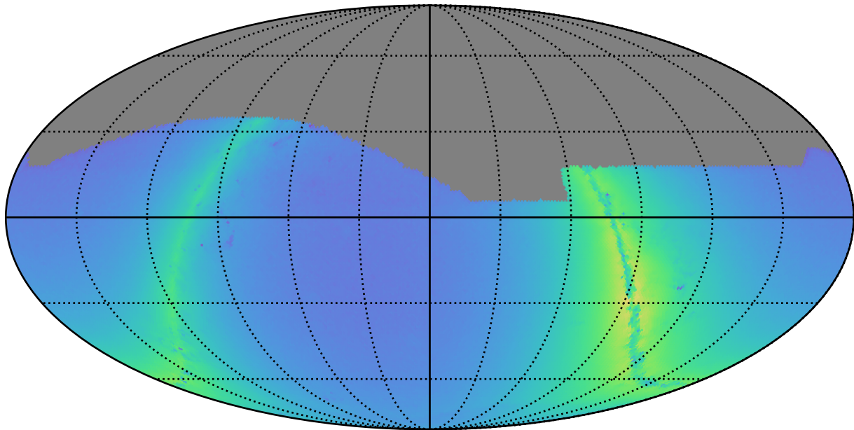
ddf_acor_sf10_lsf20_lsr20_v3.4_10yrs r: Nstars_no_crowding
