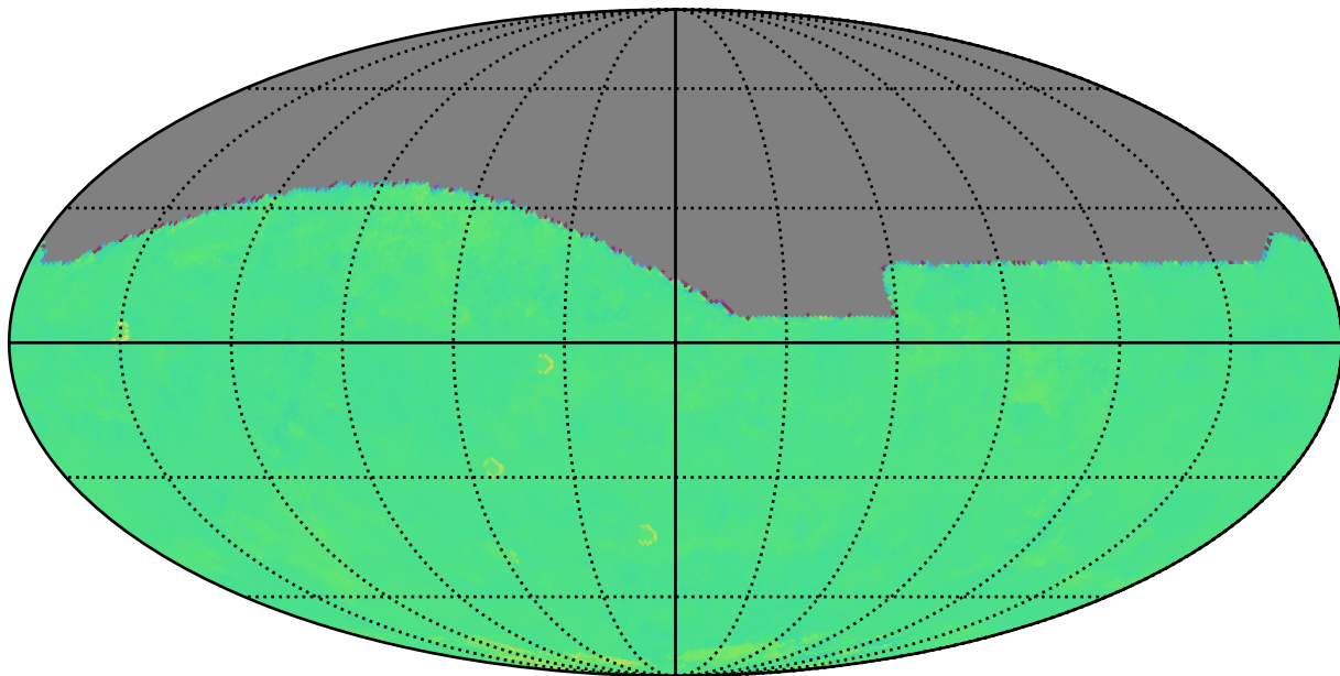
ddf_acor_sf10_lsf20_lsr20_v3.4_10yrs r: Kuiper rotTelPos
