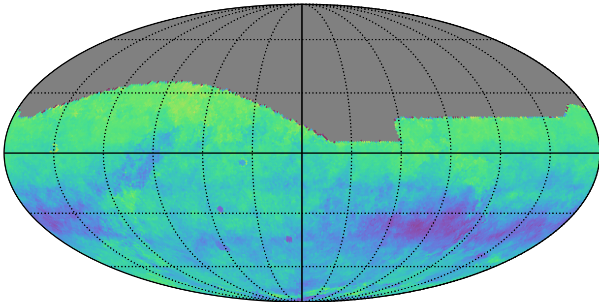
ddf_acor_sf10_lsf20_lsr20_v3.4_10yrs r: Kuiper rotSkyPos
