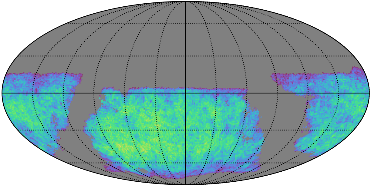
ddf_acor_sf10_lsf20_lsr20_v3.4_10yrs i band non-DD year 1: ExgalM5WithCuts
