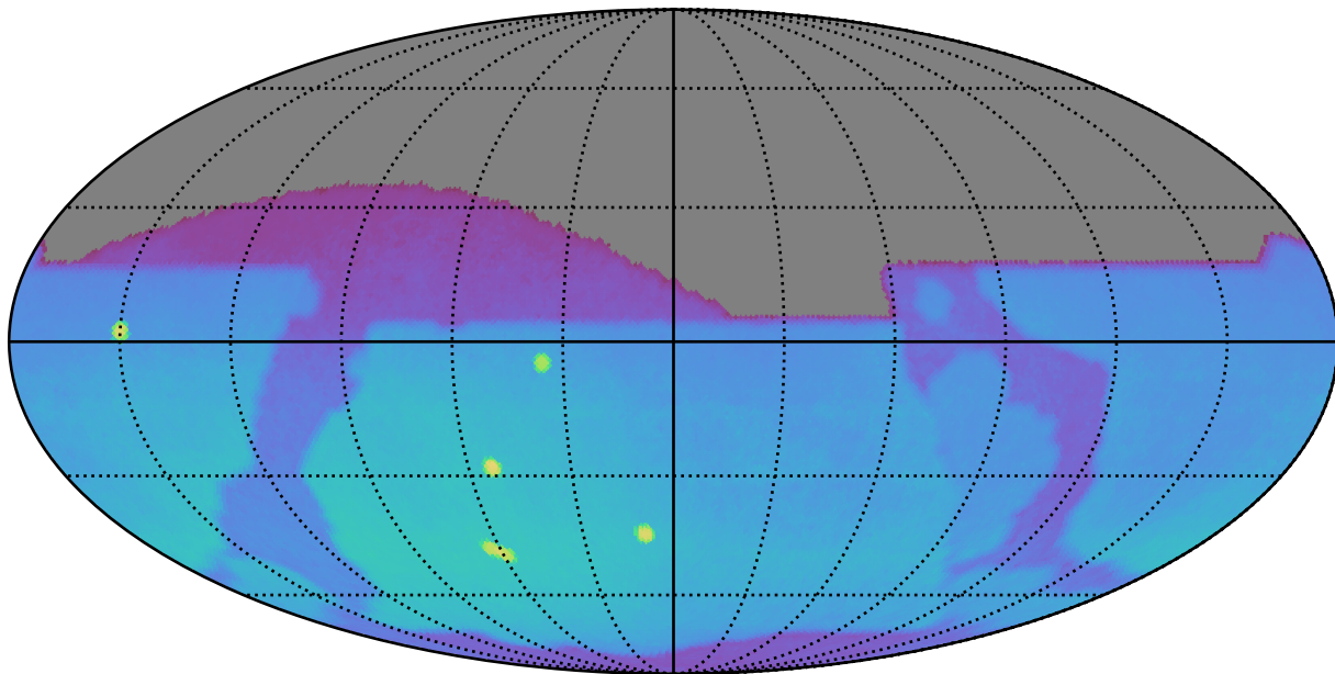
ddf_acor_sf10_lsf20_lsr20_v3.4_10yrs : Brown Dwarf, L7
