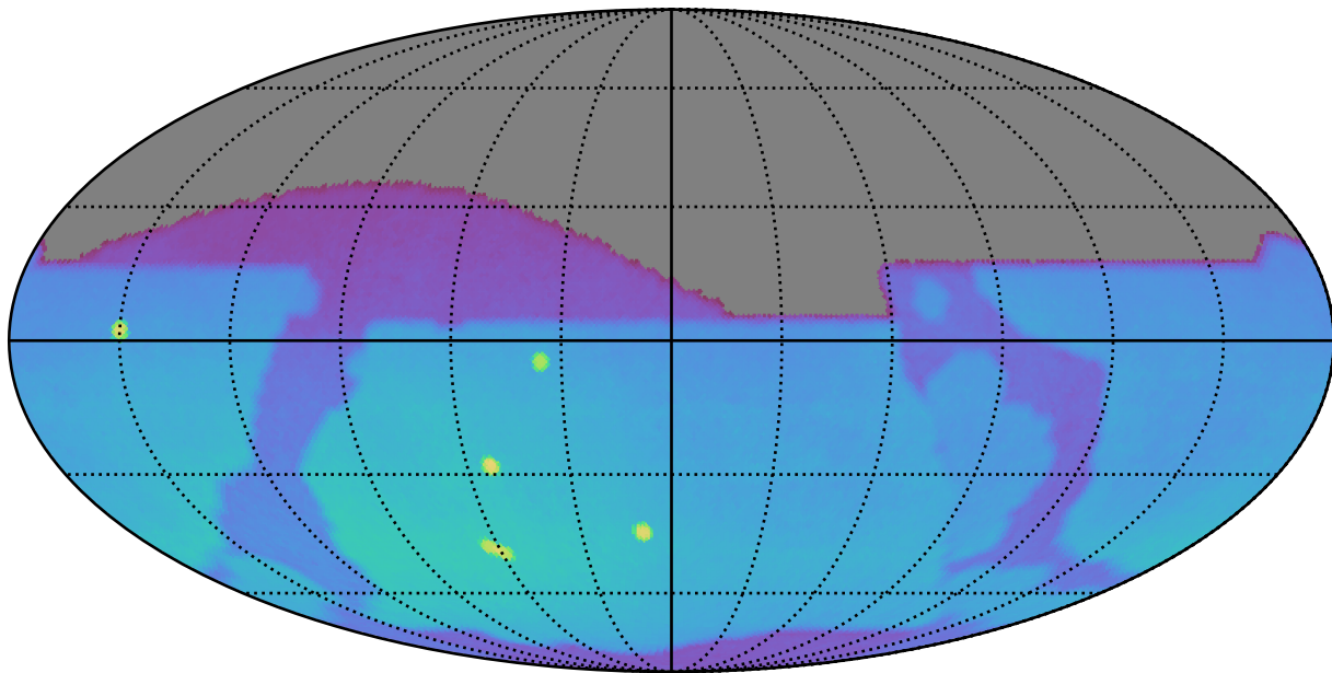
ddf_acor_sf10_lsf20_lsr20_v3.4_10yrs : Brown Dwarf, L4
