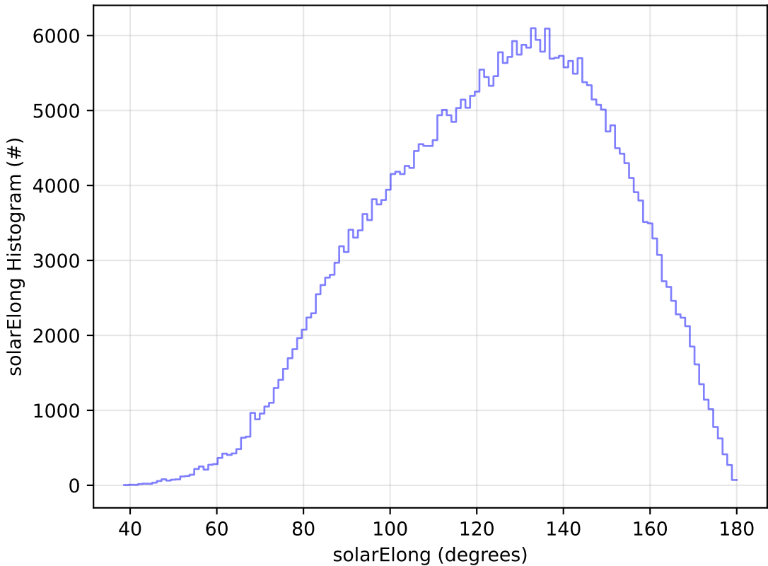
ddf_acor_sf10_lsf20_lsr20_v3.4_10yrs WFD y band: solarElong Histogram
