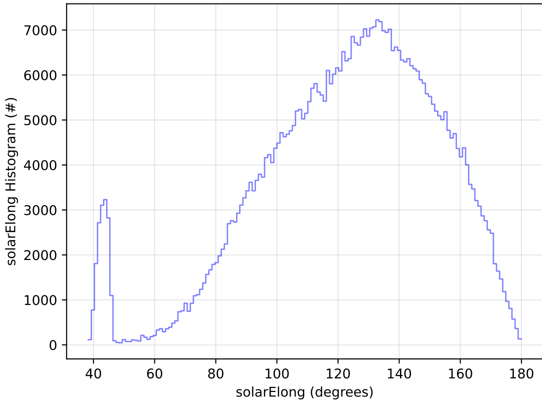
ddf_acor_sf10_lsf20_lsr20_v3.4_10yrs WFD r band: solarElong Histogram
