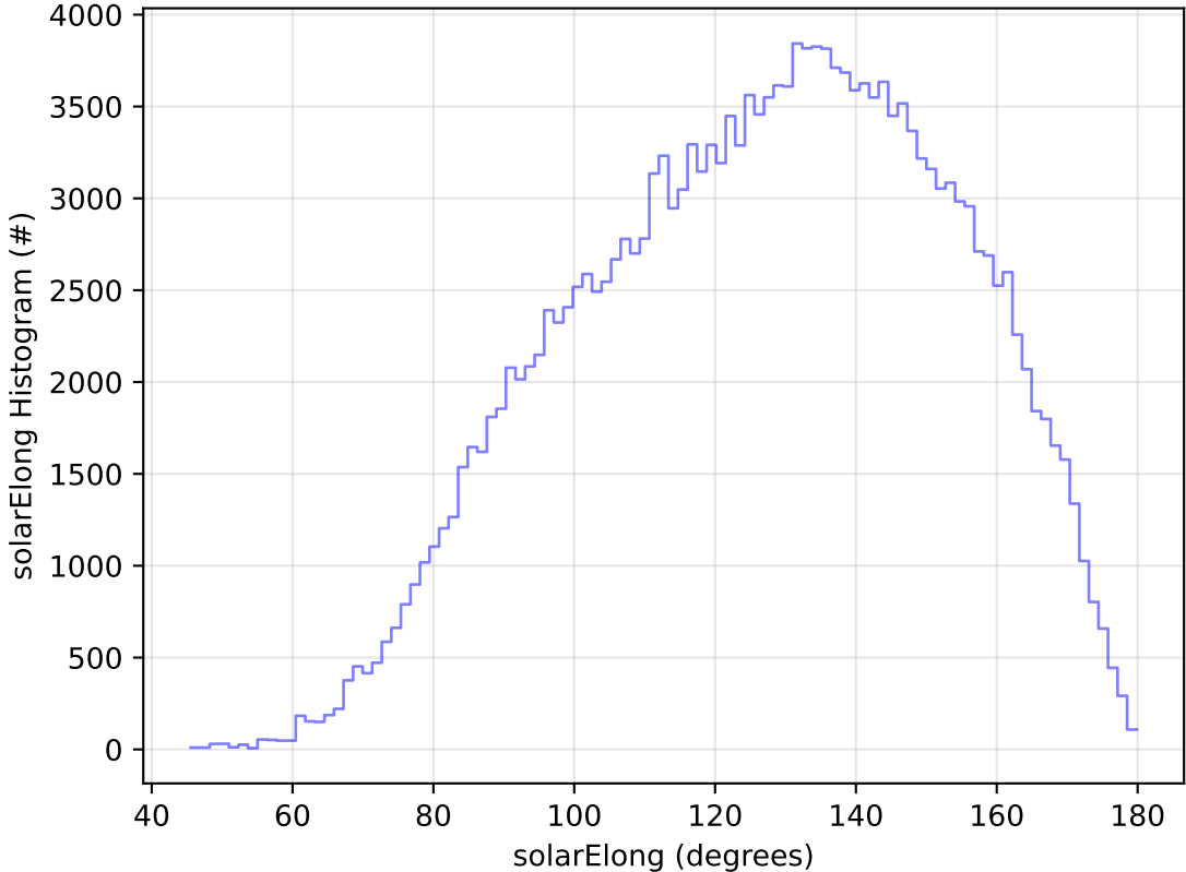
ddf_acor_sf10_lsf20_lsr20_v3.4_10yrs WFD g band: solarElong Histogram
