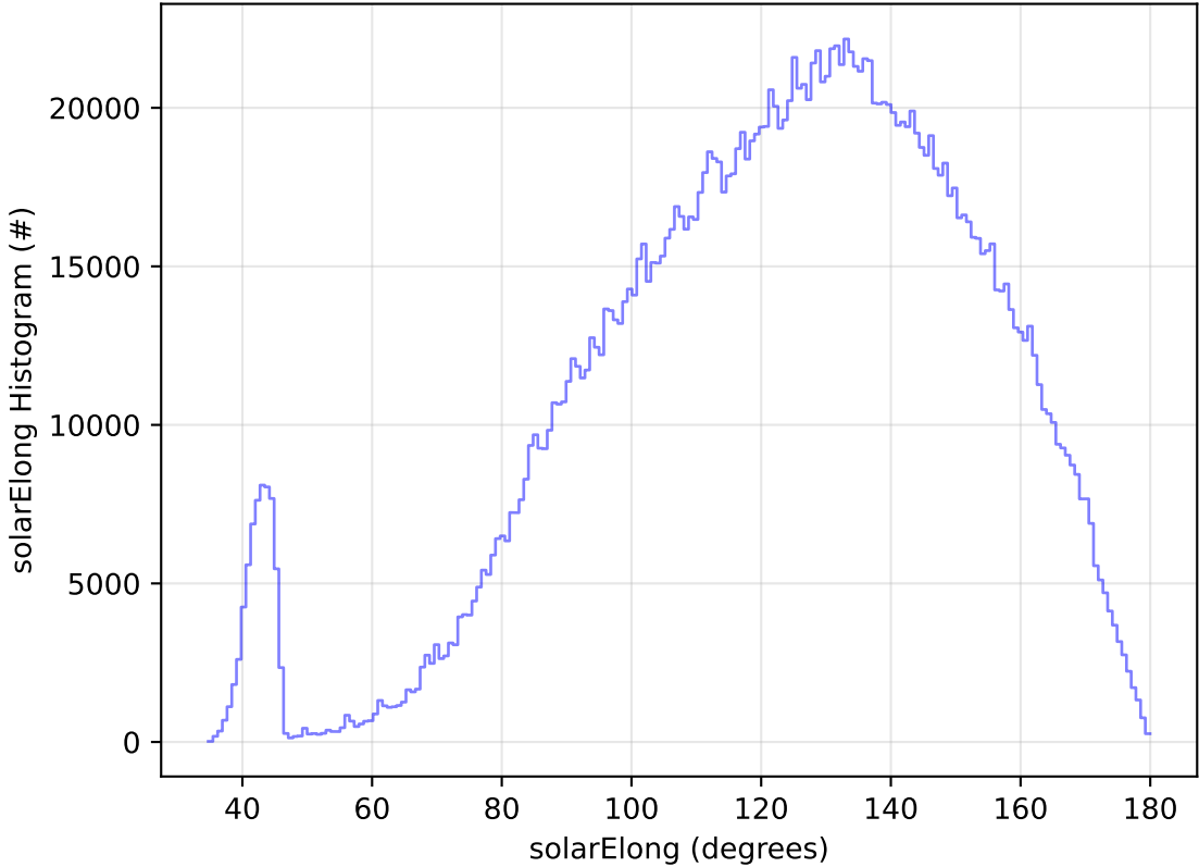
ddf_acor_sf10_lsf20_lsr20_v3.4_10yrs WFD all bands: solarElong Histogram
