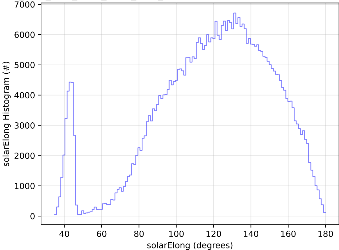
ddf_acor_sf10_lsf20_lsr20_v3.4_10yrs All sky z band: solarElong Histogram
