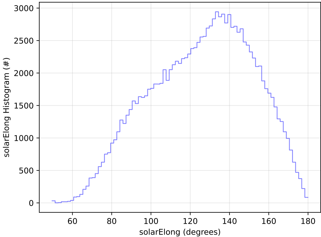
ddf_acor_sf10_lsf20_lsr20_v3.4_10yrs All sky u band: solarElong Histogram
