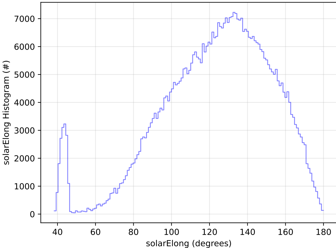
ddf_acor_sf10_lsf20_lsr20_v3.4_10yrs All sky r band: solarElong Histogram
