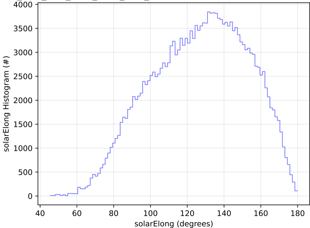
ddf_acor_sf10_lsf20_lsr20_v3.4_10yrs All sky g band: solarElong Histogram
