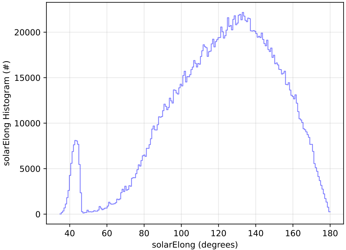
ddf_acor_sf10_lsf20_lsr20_v3.4_10yrs All sky all bands: solarElong Histogram
