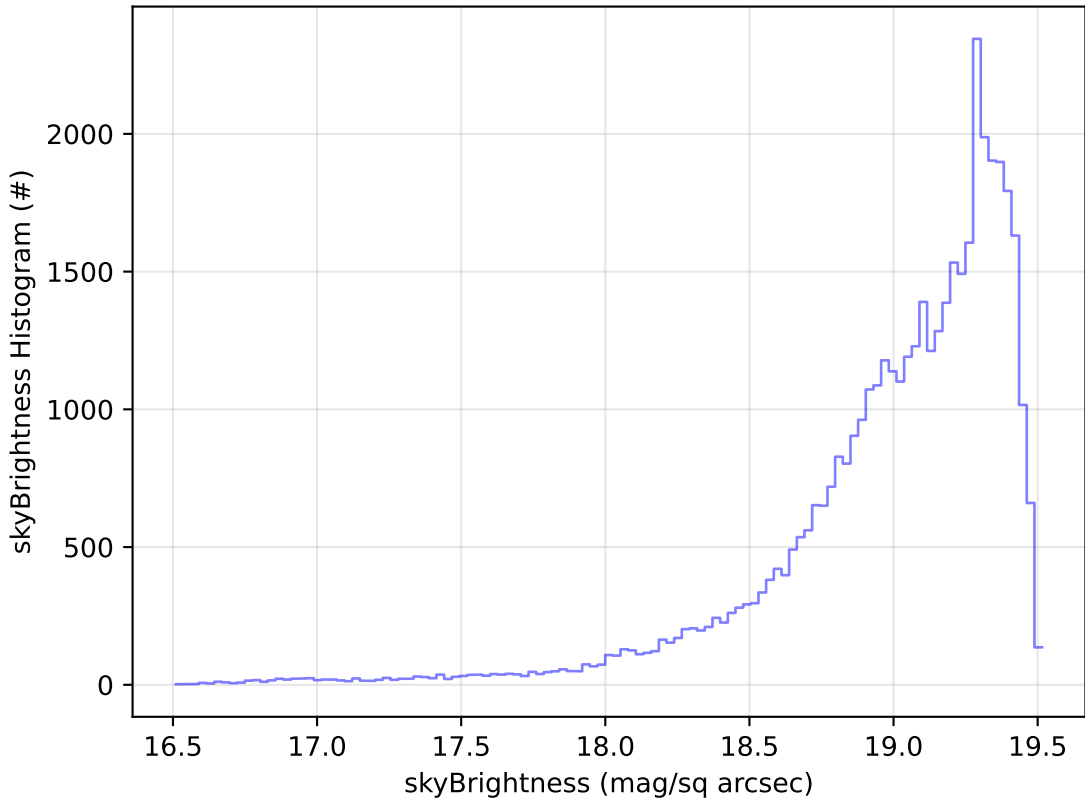
ddf_acor_sf10_lsf20_lsr20_v3.4_10yrs Yr 1 z band: skyBrightness Histogram
