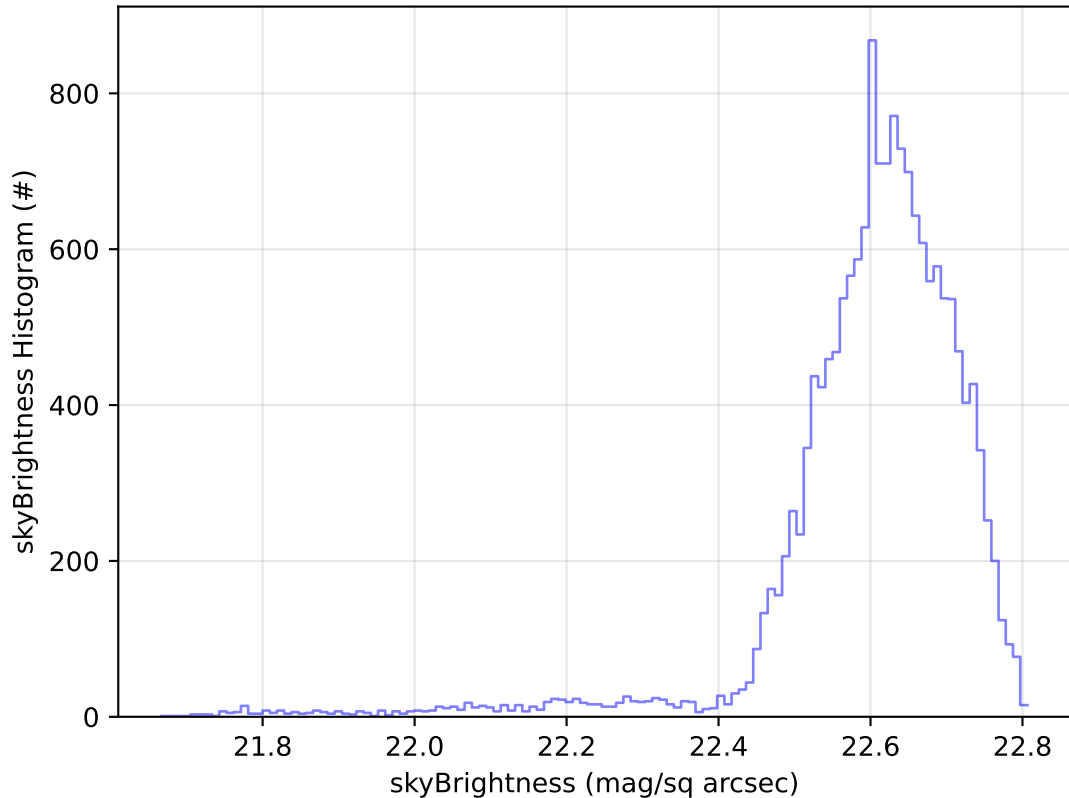
ddf_acor_sf10_lsf20_lsr20_v3.4_10yrs Yr 1 u band: skyBrightness Histogram
