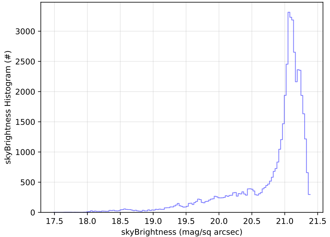
ddf_acor_sf10_lsf20_lsr20_v3.4_10yrs Yr 1 r band: skyBrightness Histogram
