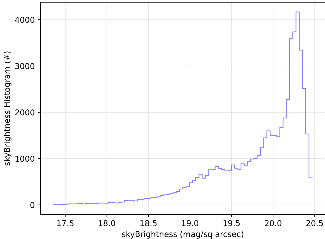
ddf_acor_sf10_lsf20_lsr20_v3.4_10yrs Yr 1 i band: skyBrightness Histogram
