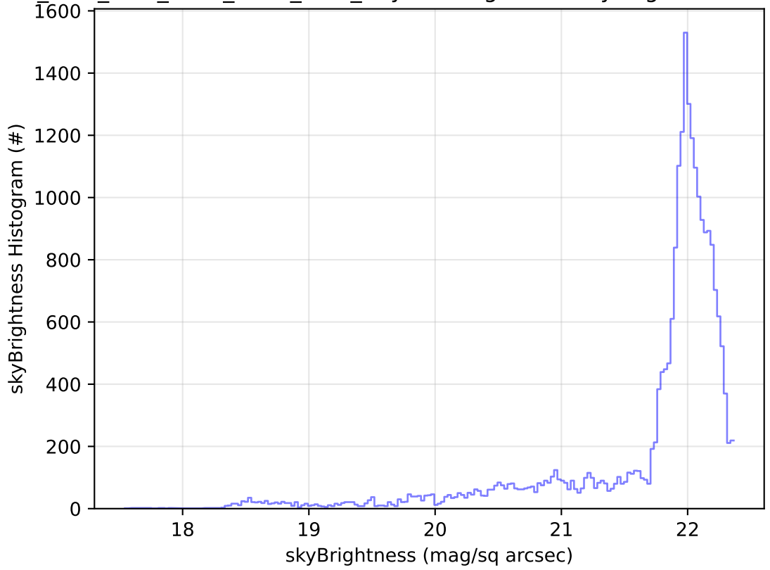
ddf_acor_sf10_lsf20_lsr20_v3.4_10yrs Yr 1 g band: skyBrightness Histogram
