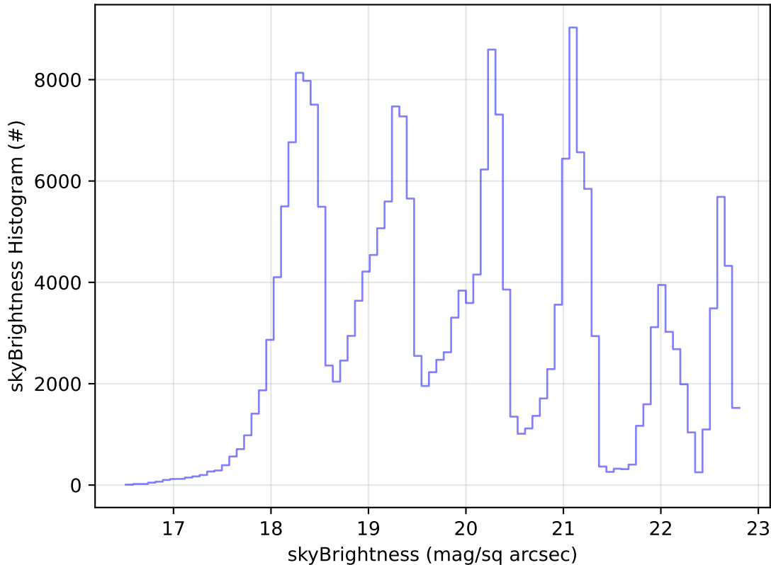
ddf_acor_sf10_lsf20_lsr20_v3.4_10yrs Yr 1 all bands: skyBrightness Histogram
