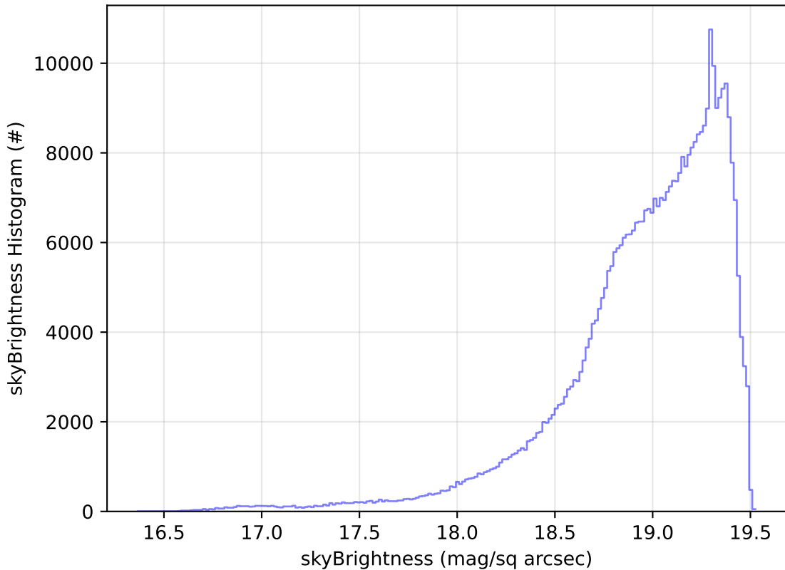
ddf_acor_sf10_lsf20_lsr20_v3.4_10yrs WFD z band: skyBrightness Histogram
