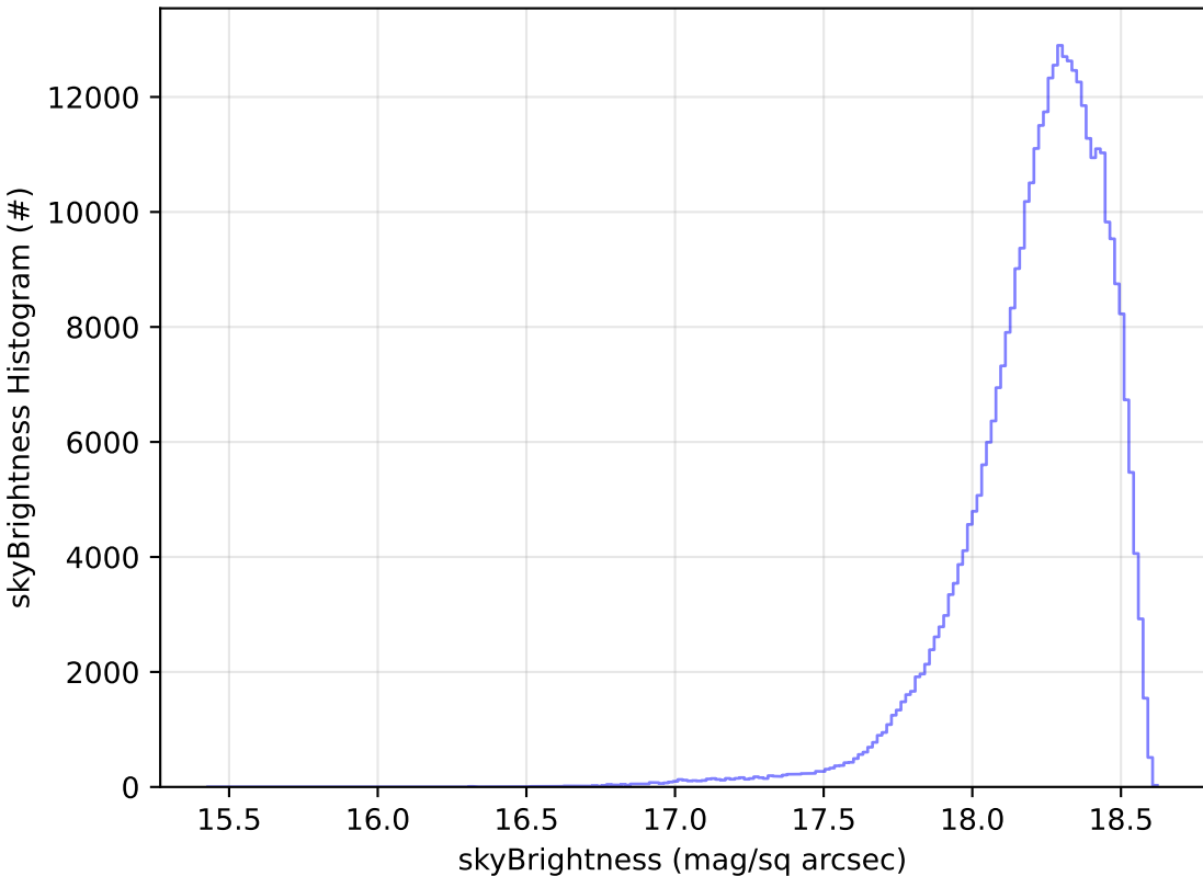
ddf_acor_sf10_lsf20_lsr20_v3.4_10yrs WFD y band: skyBrightness Histogram
