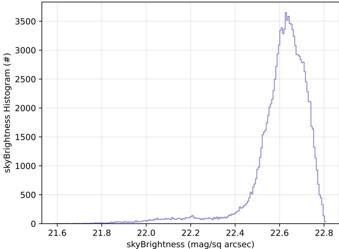
ddf_acor_sf10_lsf20_lsr20_v3.4_10yrs WFD u band: skyBrightness Histogram
