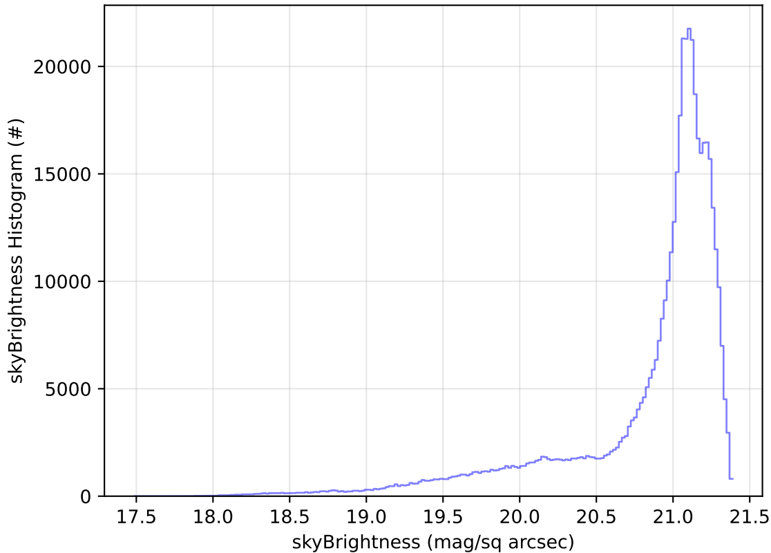
ddf_acor_sf10_lsf20_lsr20_v3.4_10yrs WFD r band: skyBrightness Histogram
