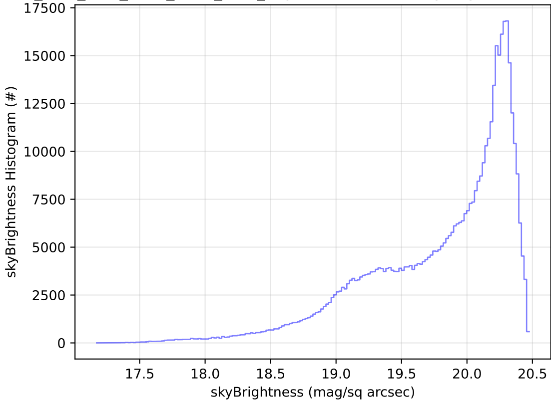
ddf_acor_sf10_lsf20_lsr20_v3.4_10yrs WFD i band: skyBrightness Histogram
