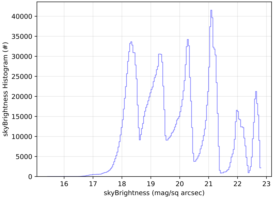
ddf_acor_sf10_lsf20_lsr20_v3.4_10yrs WFD all bands: skyBrightness Histogram
