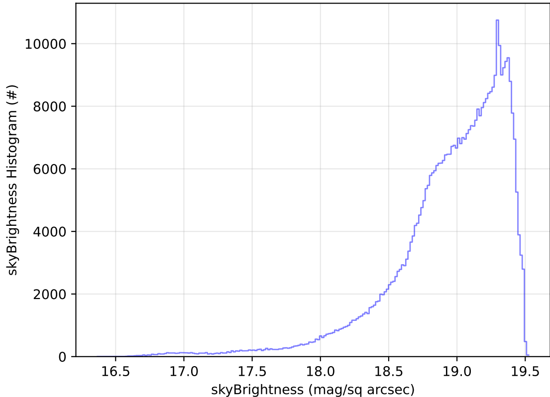
ddf_acor_sf10_lsf20_lsr20_v3.4_10yrs All sky z band: skyBrightness Histogram
