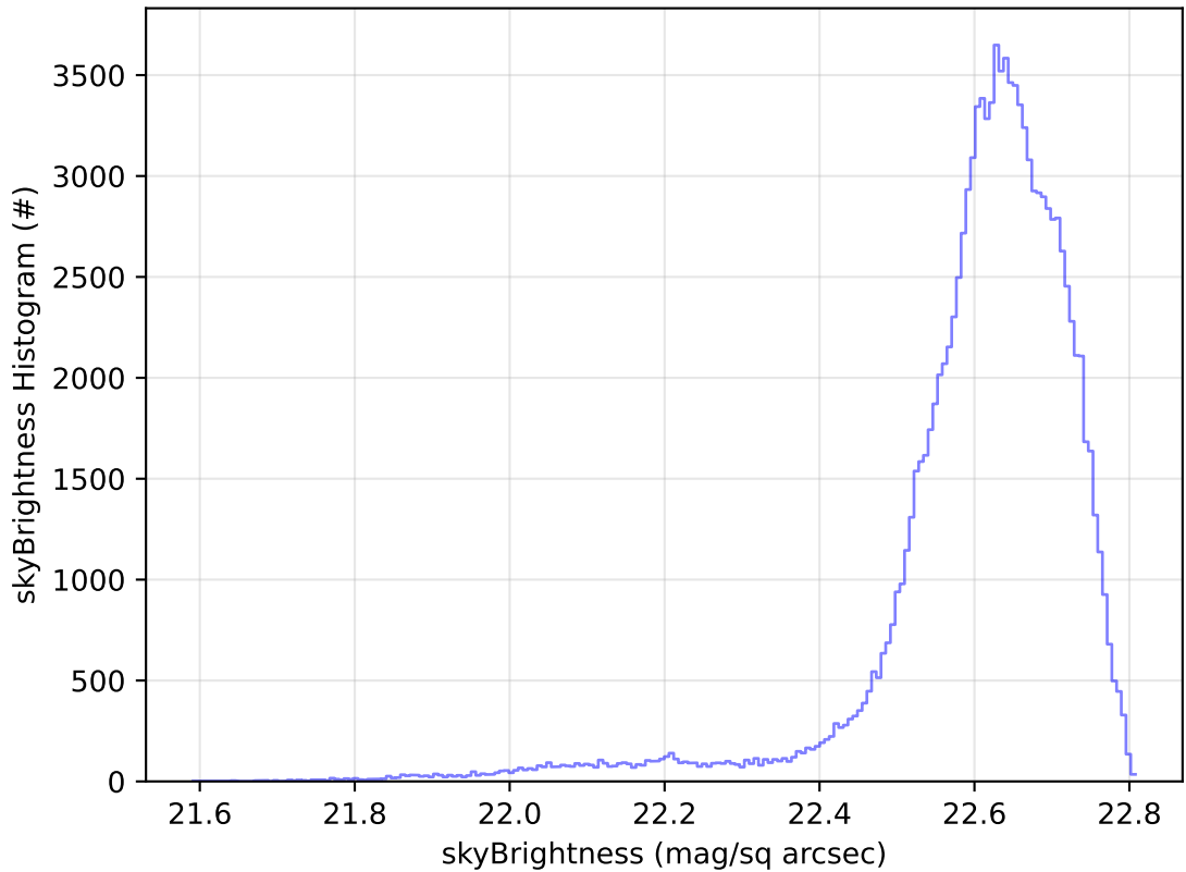
ddf_acor_sf10_lsf20_lsr20_v3.4_10yrs All sky u band: skyBrightness Histogram
