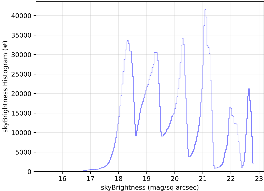
ddf_acor_sf10_lsf20_lsr20_v3.4_10yrs All sky all bands: skyBrightness Histogram
