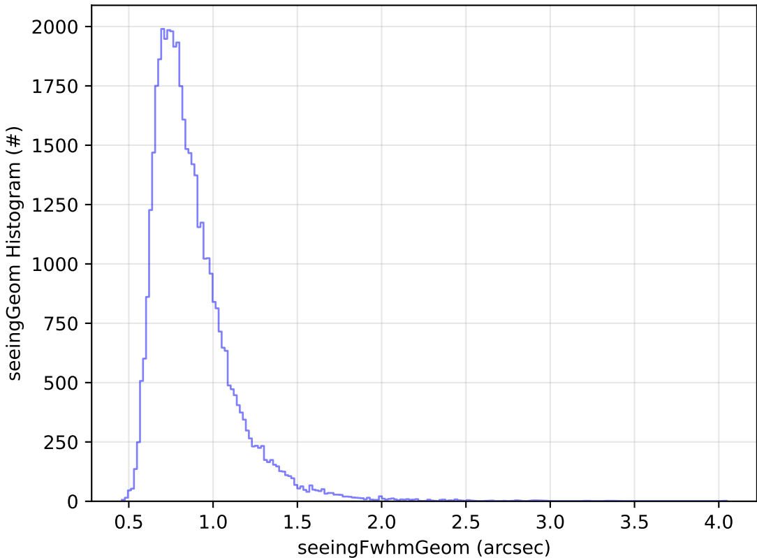
ddf_acor_sf10_lsf20_lsr20_v3.4_10yrs Yr 1 z band: seeingGeom Histogram
