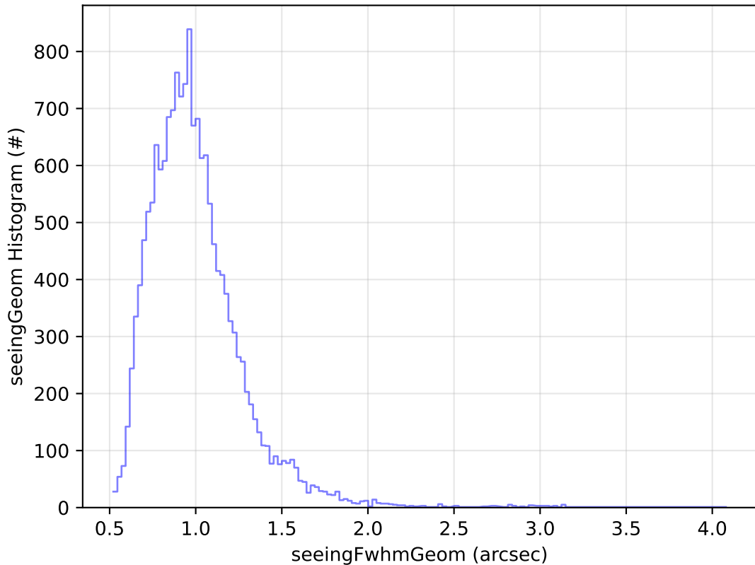
ddf_acor_sf10_lsf20_lsr20_v3.4_10yrs Yr 1 u band: seeingGeom Histogram
