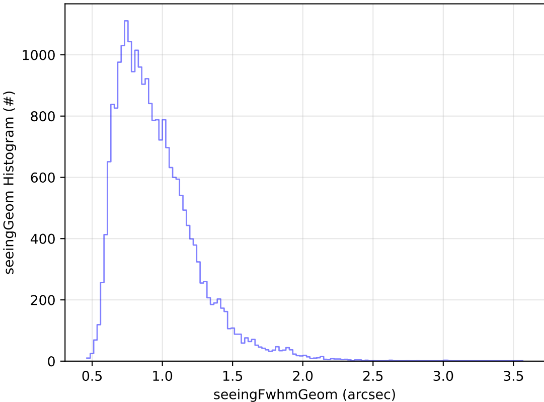
ddf_acor_sf10_lsf20_lsr20_v3.4_10yrs Yr 1 g band: seeingGeom Histogram
