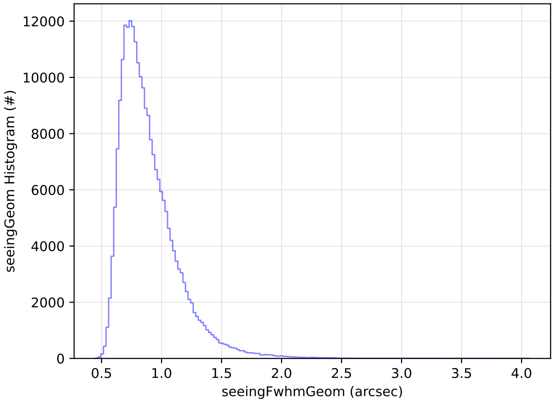
ddf_acor_sf10_lsf20_lsr20_v3.4_10yrs Yr 1 all bands: seeingGeom Histogram
