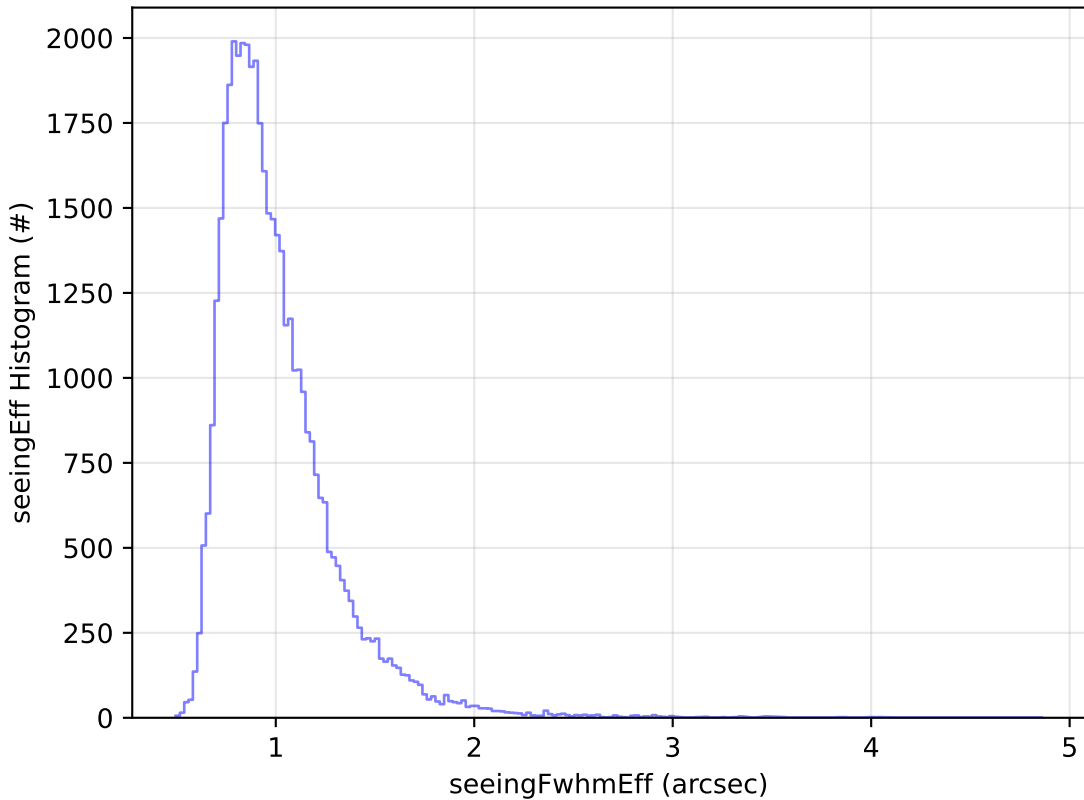
ddf_acor_sf10_lsf20_lsr20_v3.4_10yrs Yr 1 z band: seeingEff Histogram
