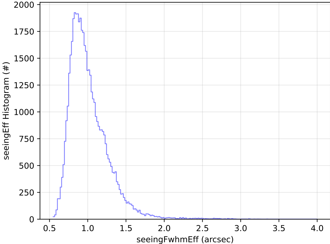
ddf_acor_sf10_lsf20_lsr20_v3.4_10yrs Yr 1 y band: seeingEff Histogram
