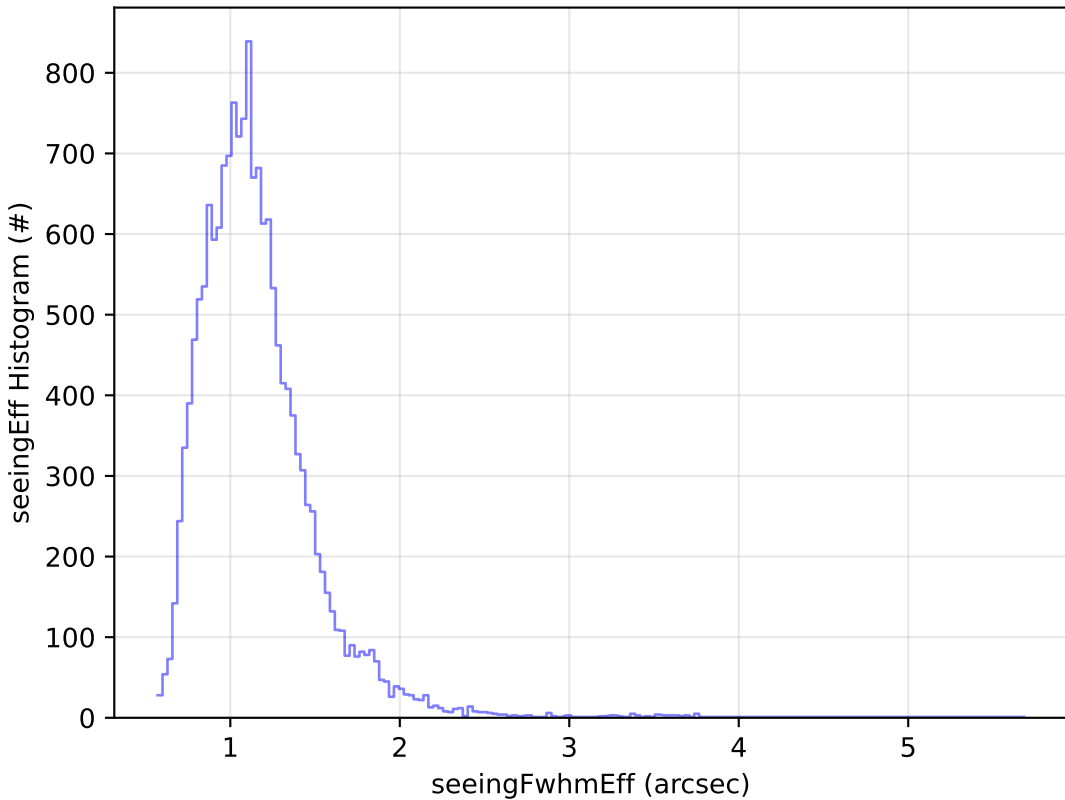
ddf_acor_sf10_lsf20_lsr20_v3.4_10yrs Yr 1 u band: seeingEff Histogram
