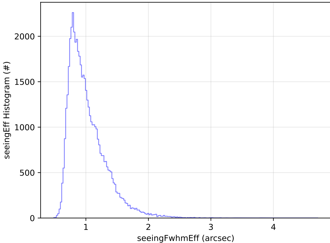
ddf_acor_sf10_lsf20_lsr20_v3.4_10yrs Yr 1 r band: seeingEff Histogram
