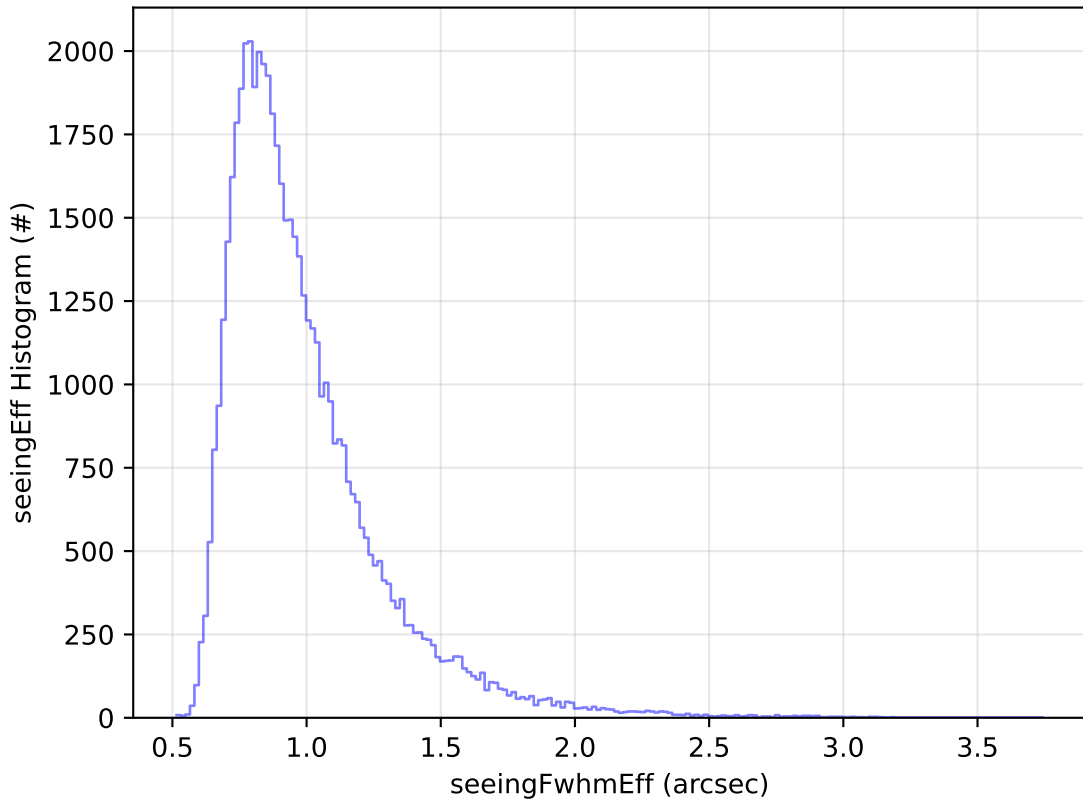
ddf_acor_sf10_lsf20_lsr20_v3.4_10yrs Yr 1 i band: seeingEff Histogram
