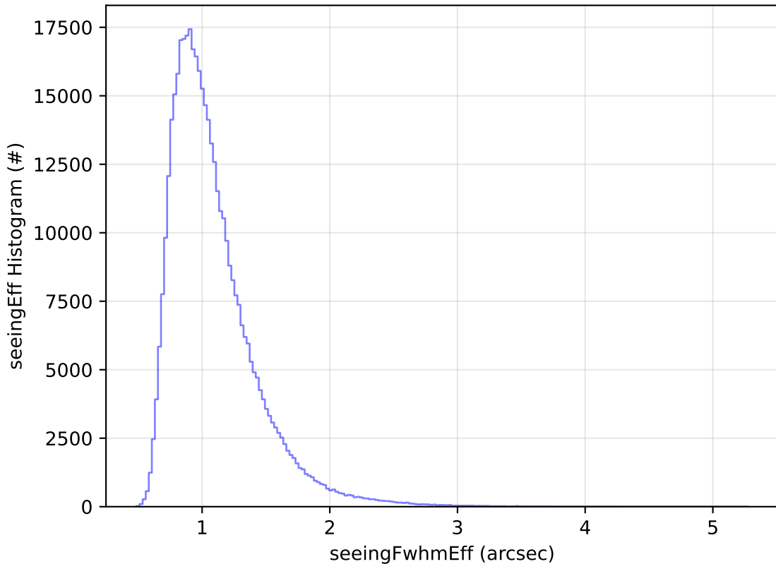
ddf_acor_sf10_lsf20_lsr20_v3.4_10yrs WFD z band: seeingEff Histogram
