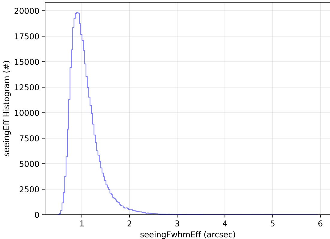
ddf_acor_sf10_lsf20_lsr20_v3.4_10yrs WFD y band: seeingEff Histogram
