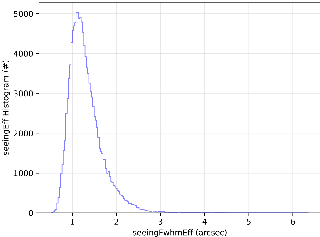
ddf_acor_sf10_lsf20_lsr20_v3.4_10yrs WFD u band: seeingEff Histogram
