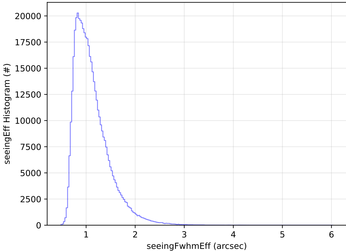
ddf_acor_sf10_lsf20_lsr20_v3.4_10yrs WFD r band: seeingEff Histogram
