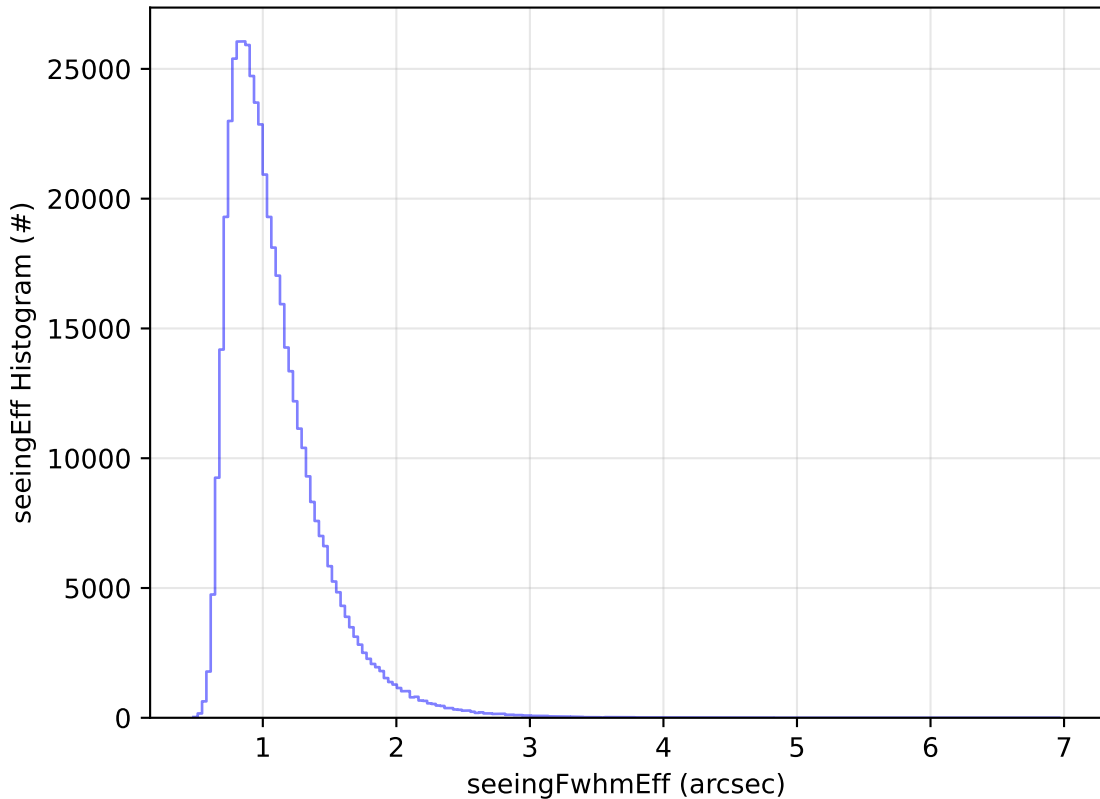
ddf_acor_sf10_lsf20_lsr20_v3.4_10yrs WFD i band: seeingEff Histogram
