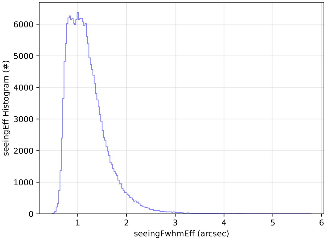
ddf_acor_sf10_lsf20_lsr20_v3.4_10yrs WFD g band: seeingEff Histogram
