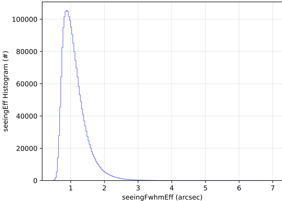
ddf_acor_sf10_lsf20_lsr20_v3.4_10yrs WFD all bands: seeingEff Histogram
